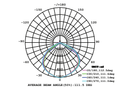
LUMINOUS INTENSITY DISTRIBUTION DIAGRAM
